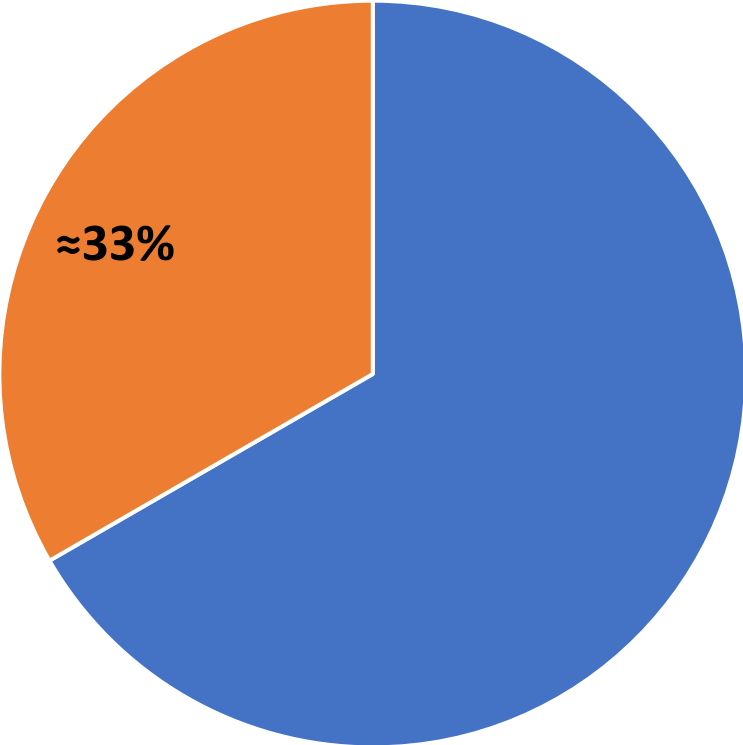
Global Green House Gas Emissions
