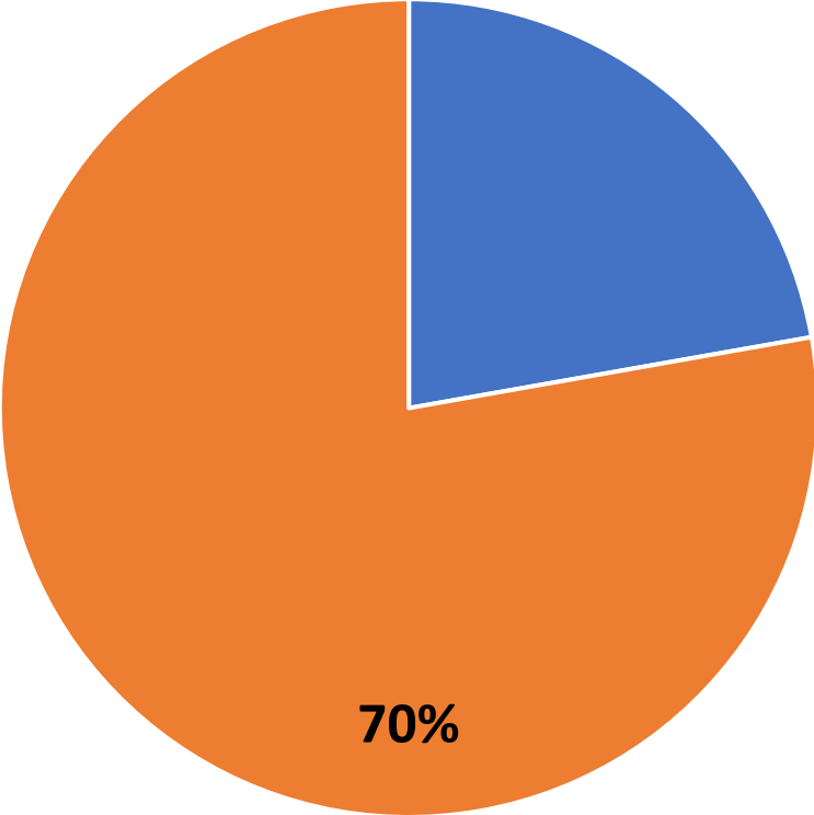
Terrestrial Biodiversity Loss
